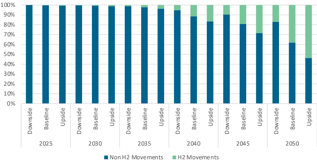
Figure 44: Split between H2 and Non H2 movements at Heathrow Airport
