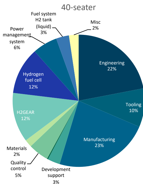
Figure 23: Breakdown of operating costs for the 40-seater
