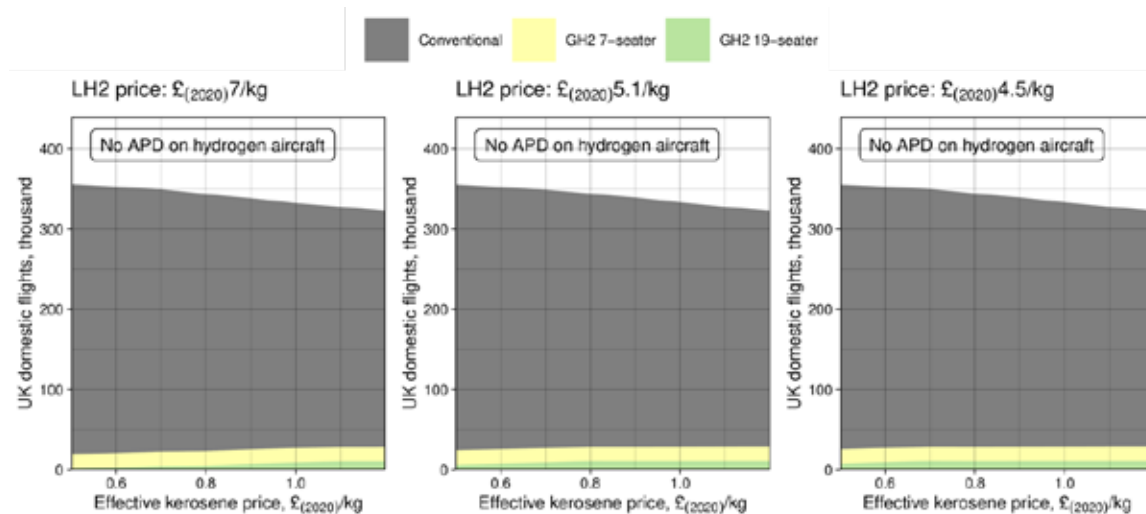
Figure 16: 7- and 19-seater gaseous hydrogen aircraft uptake (flights) in the UK domestic aviation system under Year-2025 Use Case A conditions across a range of kerosene and hydrogen prices.
