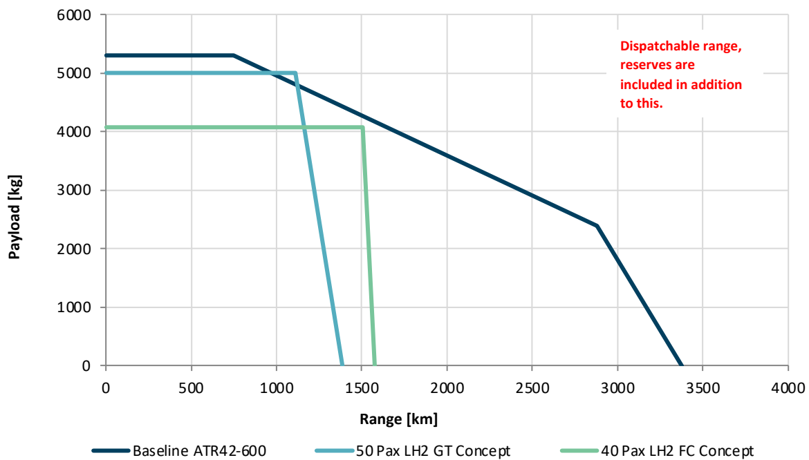
Figure 22: Payload Range Diagram of the Use Case B aircraft concepts
