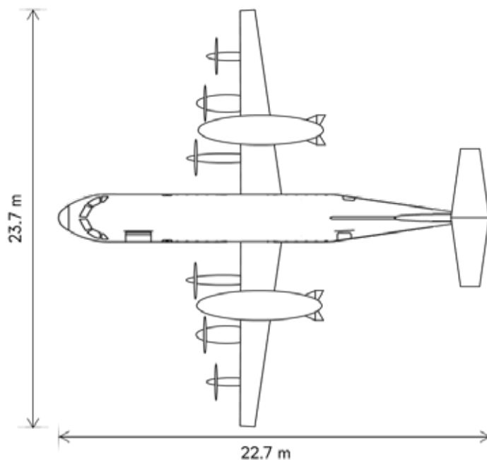
Figure 21: NAPKIN 50 seat gas turbine aircraft
