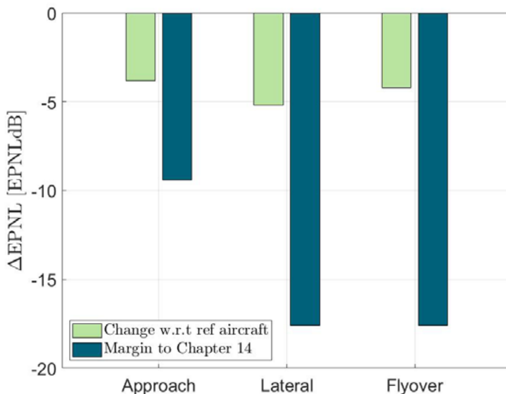
Figure 28: GKN 40 seat margins to noise limits set by Chapter 14 and changes in levels relative to baseline aircraft.
