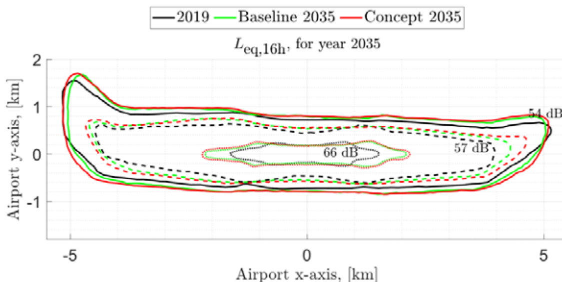
Figure 34: Contour calculation for 2035. Results are compared to the published contours for LCY in 2019 and a baseline calculation for year 2035 assuming no hydrogen aircraft introduction. Line types indicate different contour levels
