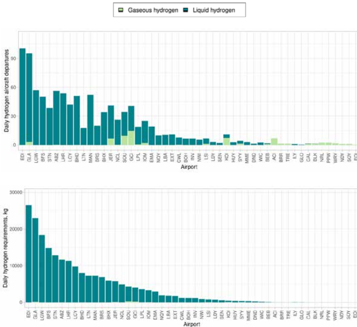
Figure 43: Airport-level number of hydrogen aircraft flights and amount of hydrogen required, for central fuel prices modelled in Use Case C (Jet A + carbon: £1.5/kg; gaseous hydrogen: 1.2/kg; liquid hydrogen: £2.3/kg). Central bars are stacked rather than overlaid. Note that only domestic demand is modelled. These simulations assume LCCs would consider adoption.
