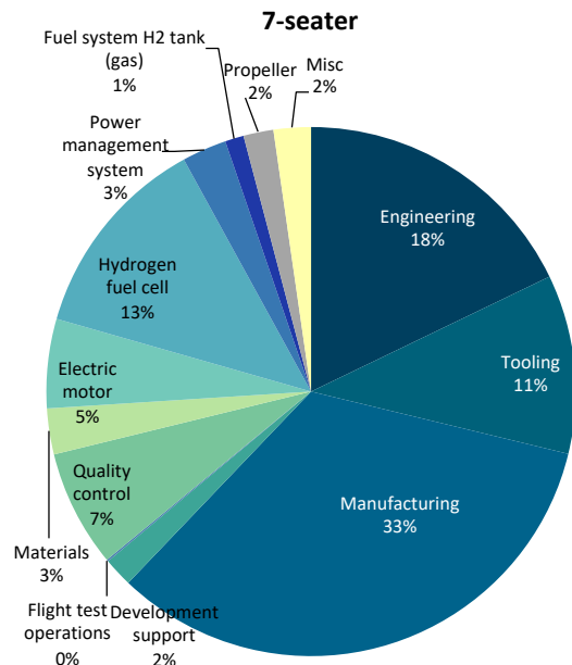
Figure 12: Breakdown of total cost of ownership of the 7-seater
