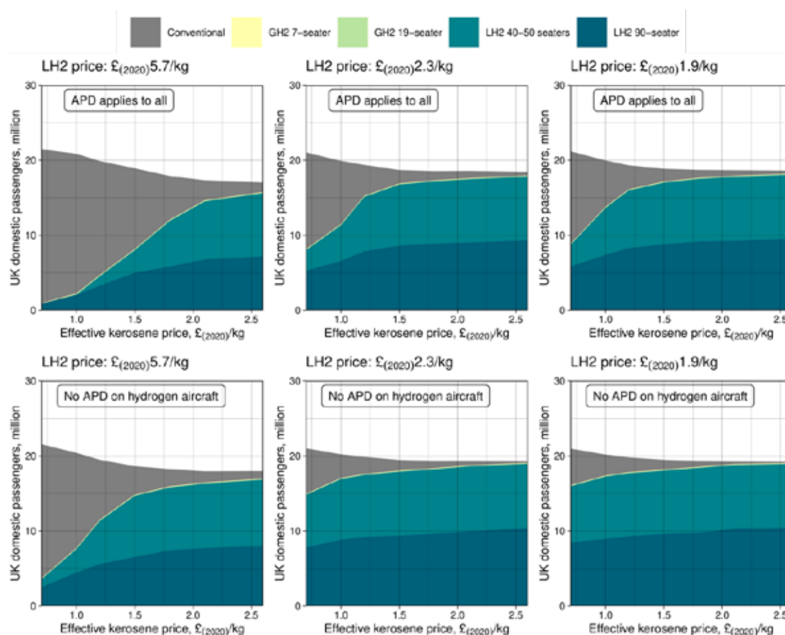
Figure 40: 7- and 19-seater gaseous hydrogen, and 40-50-seater and 90-seater liquid hydrogen aircraft, projected number of passengers in the UK domestic aviation system under Year-2040 Use Case C1 conditions across a range of kerosene and hydrogen prices. These simulations assume LCCs would consider adoption.
