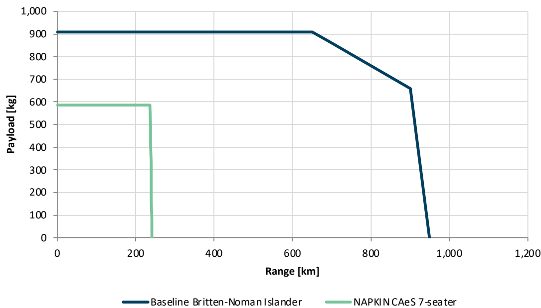
Figure 9: Payload-Range diagram of the NAPKIN 7-seater aircraft and the baseline aircraft, Britten-Norman Islander
