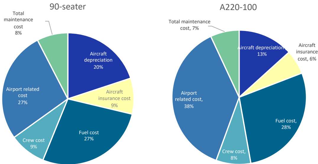
Figure 38: Breakdown of the total cost of ownership of the 90-seater (left) and the A220-100 (right)
