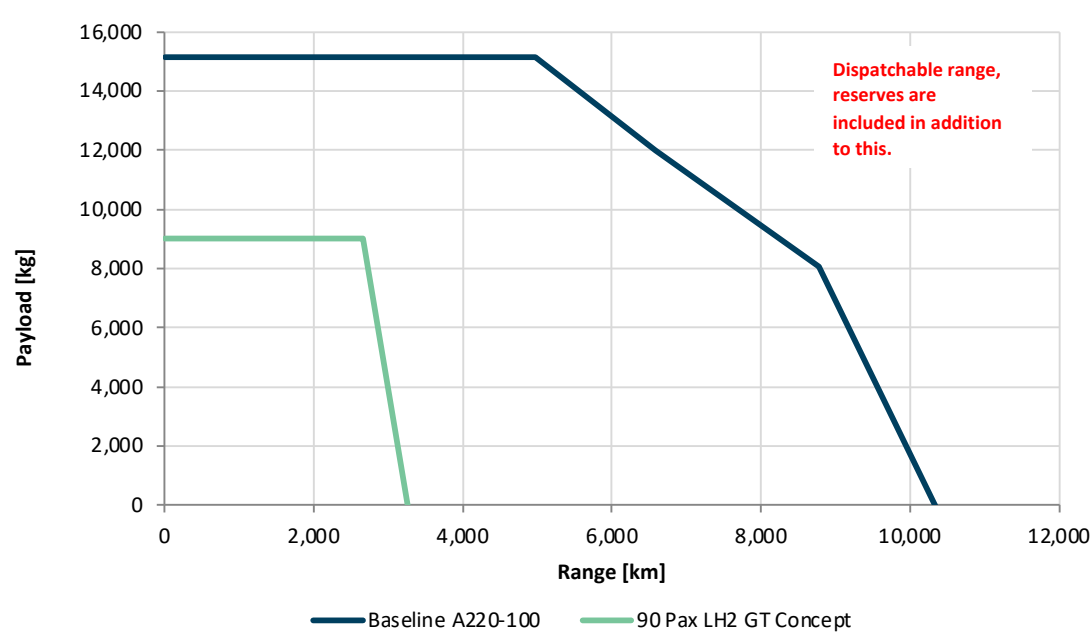
Figure 36: Payload Range diagram for the NAPKIN 90-seater
