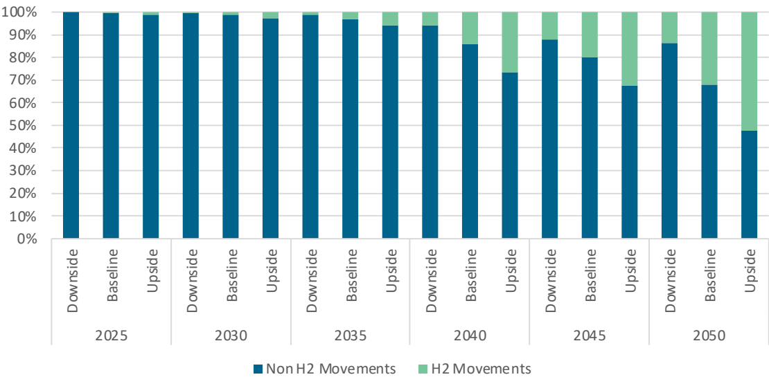
Figure 33: Split between H2 and Non H2 movements at London City Airport
