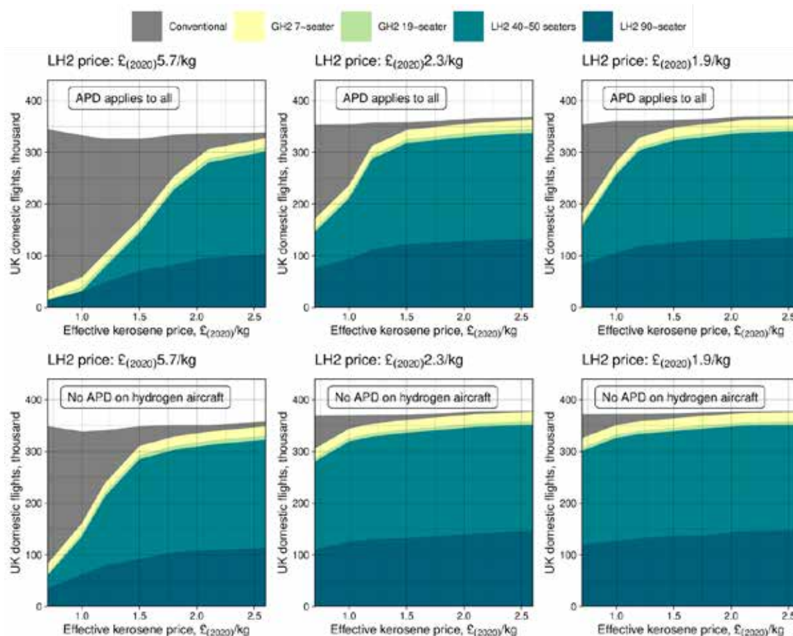
Figure 39: 7- and 19-seater gaseous hydrogen, and 40-50-seater and 90-seater liquid hydrogen aircraft projected profit-optimal number of flights in the UK domestic aviation system under Year-2040 Use Case C1 conditions across a range of kerosene and hydrogen prices. These simulations assume LCCs would consider adoption.
