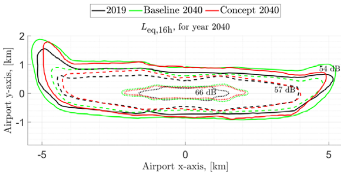
Figure 35: Contour calculation for 2040. Results are compared to the published contours for LCY in 2019 and a baseline calculation for year 2040 assuming no hydrogen aircraft introduction. Line types indicate different contour levels.
