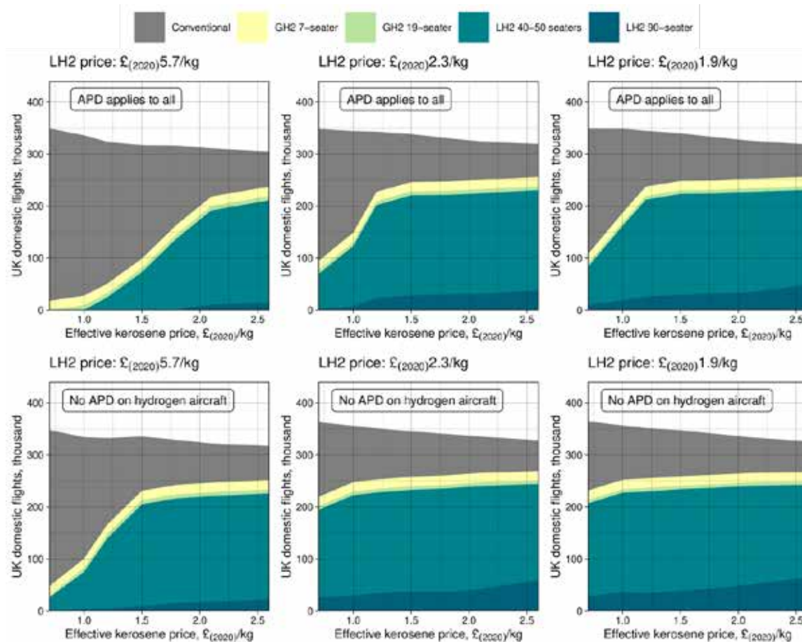
Figure 41: 7- and 19-seater gaseous hydrogen, and 40-50-seater and 90-seater liquid hydrogen aircraft, projected number of flights in the UK domestic aviation system under Year-2040 Use Case C2 conditions across a range of kerosene and hydrogen prices. These simulations assume LCCs would not consider adoption.
