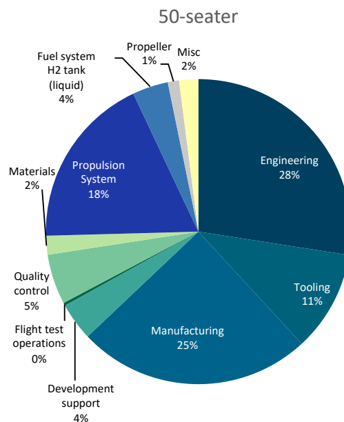
Figure 24: Breakdown of operating costs for the 50-seater
