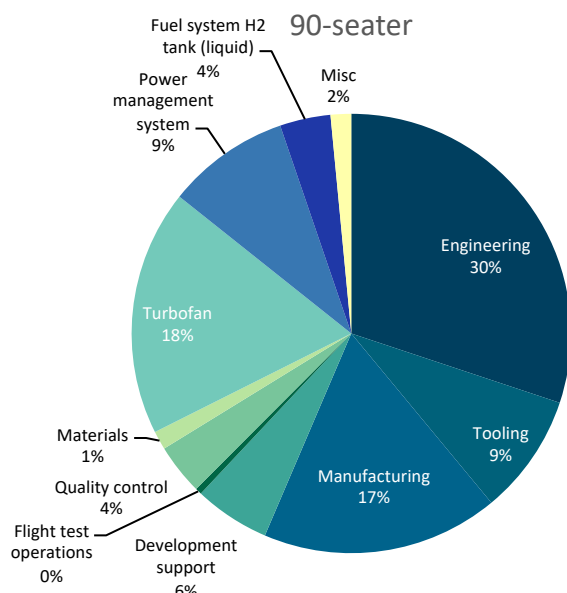
Figure 37: Breakdown of the operating costs of the 90-seater
