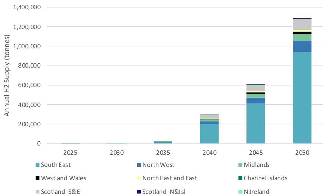
Figure 6: Regional supply of hydrogen (annual, tonnes) up to 2050 - Baseline scenario
