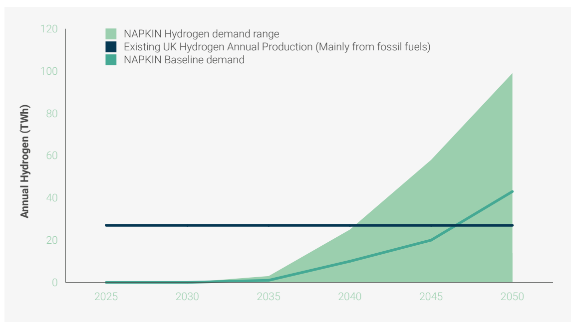
Figure 4: Comparison between NAPKIN forecast hydrogen demand with UK current hydrogen production
