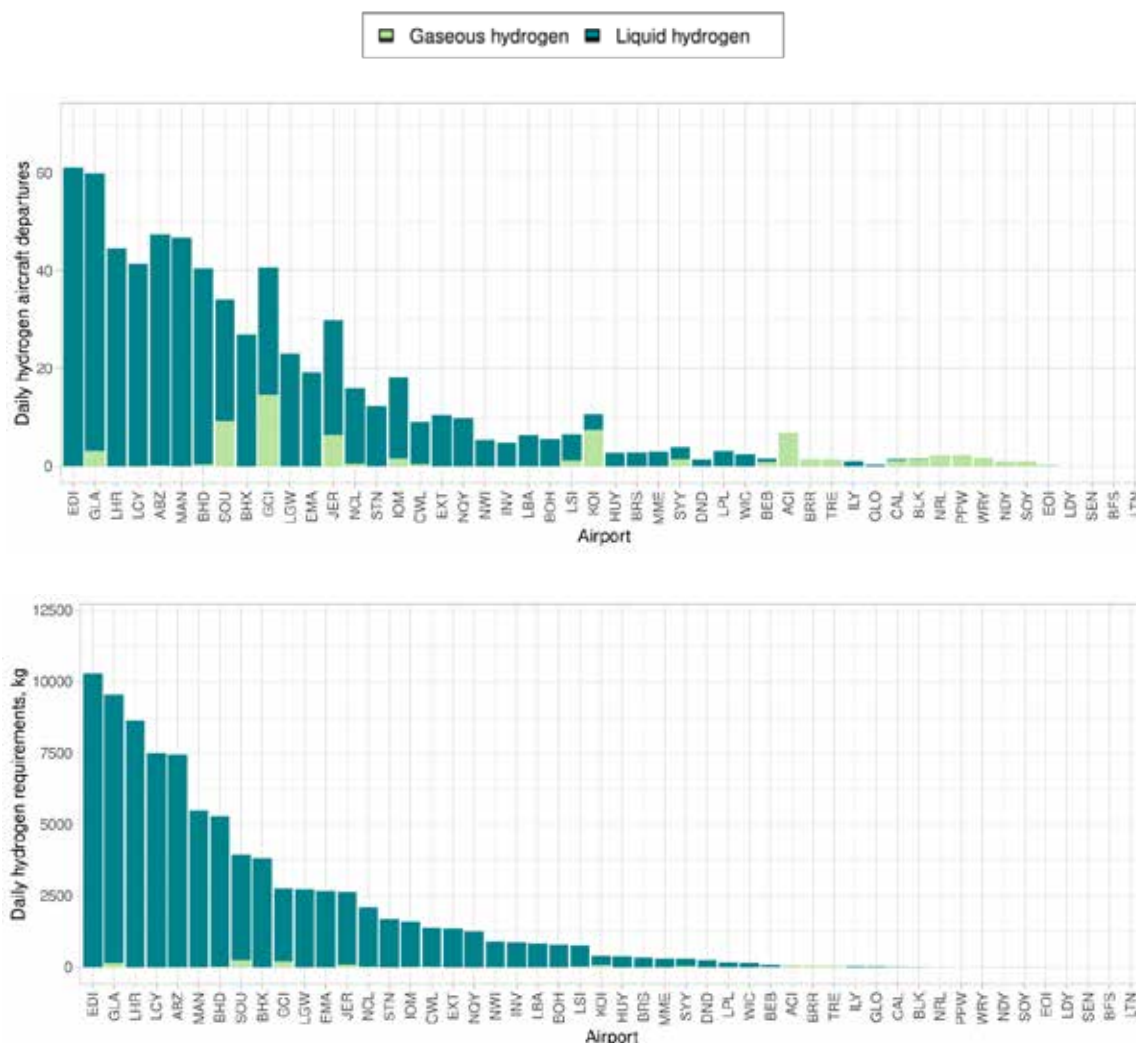
Figure 32: Airport-level number of hydrogen aircraft flights and amount of hydrogen required, at central fuel prices modelled for Use Case B (Jet A+carbon: £1.3/kg; gaseous hydrogen: £1.3/kg; liquid hydrogen: £2.6/kg). Note that only domestic demand is modelled.
